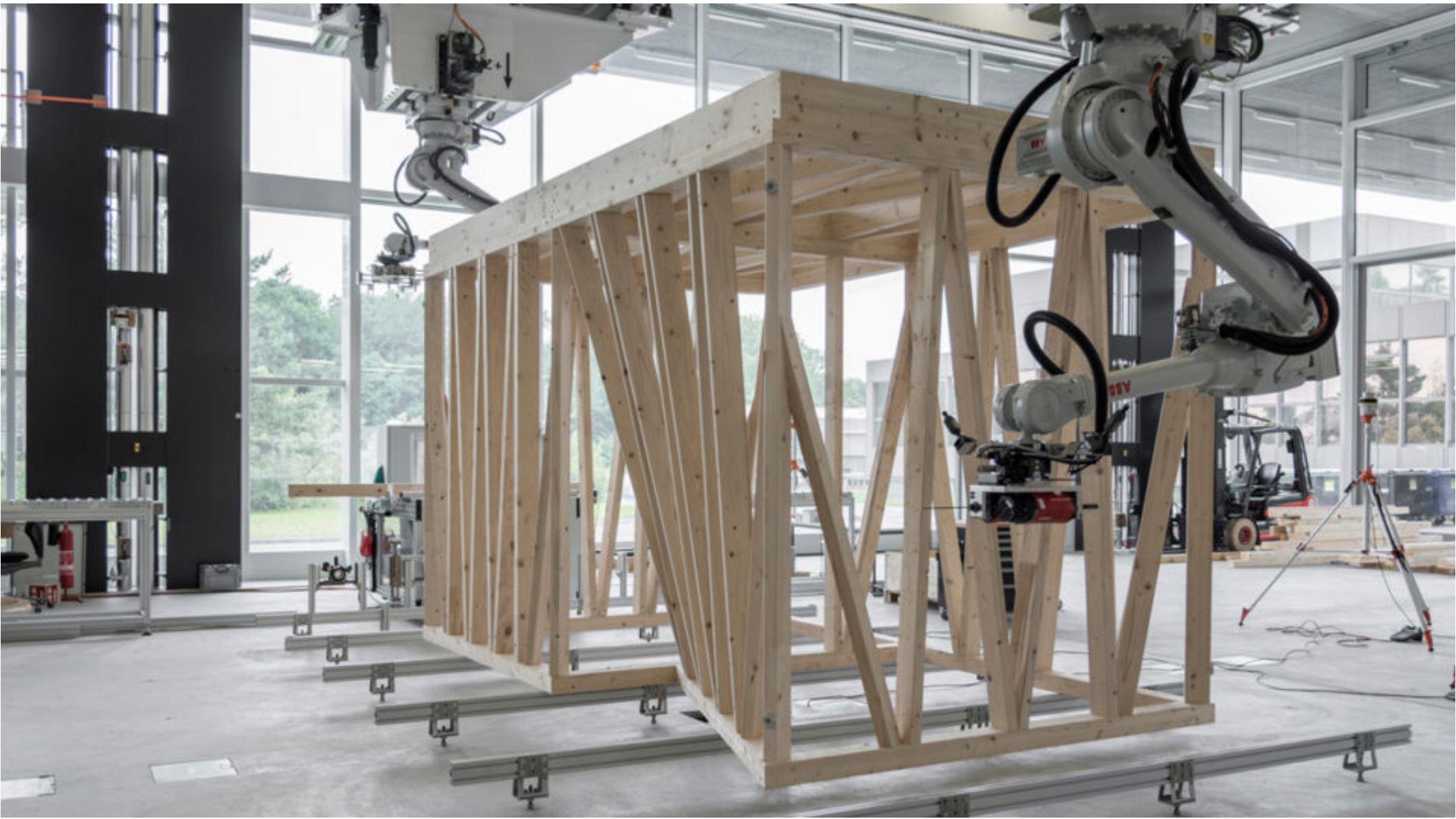
Laboratorio fabricación digital-robótica ETH Zürich, 2018 https://cdn.materialdistrict.com/wp-content/uploads/2018/05/building-with-robots-using-spatial-timber-assemblies-method-02-960x537.jpg
