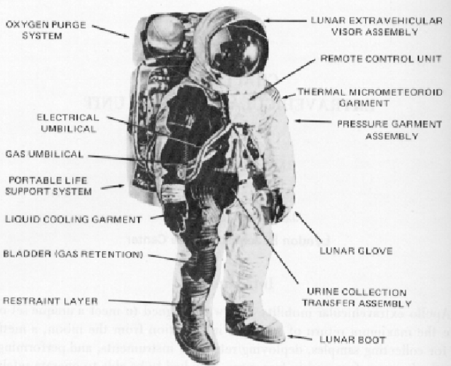
Figure 1. Cutaway of Apollo extravehicular mobility unit.
